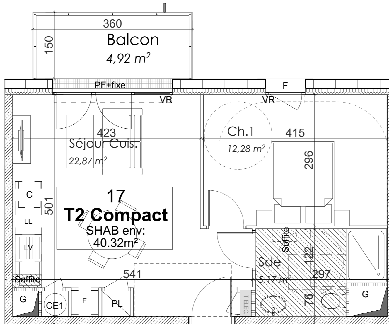
Plan 1/50
