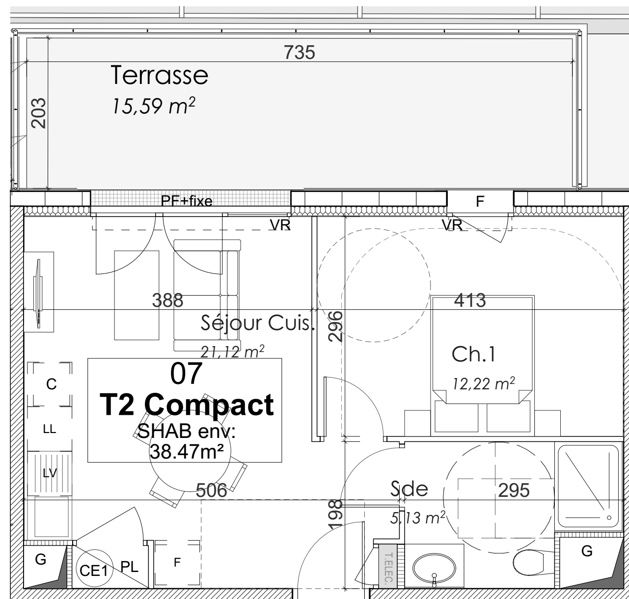
Plan 1/50
