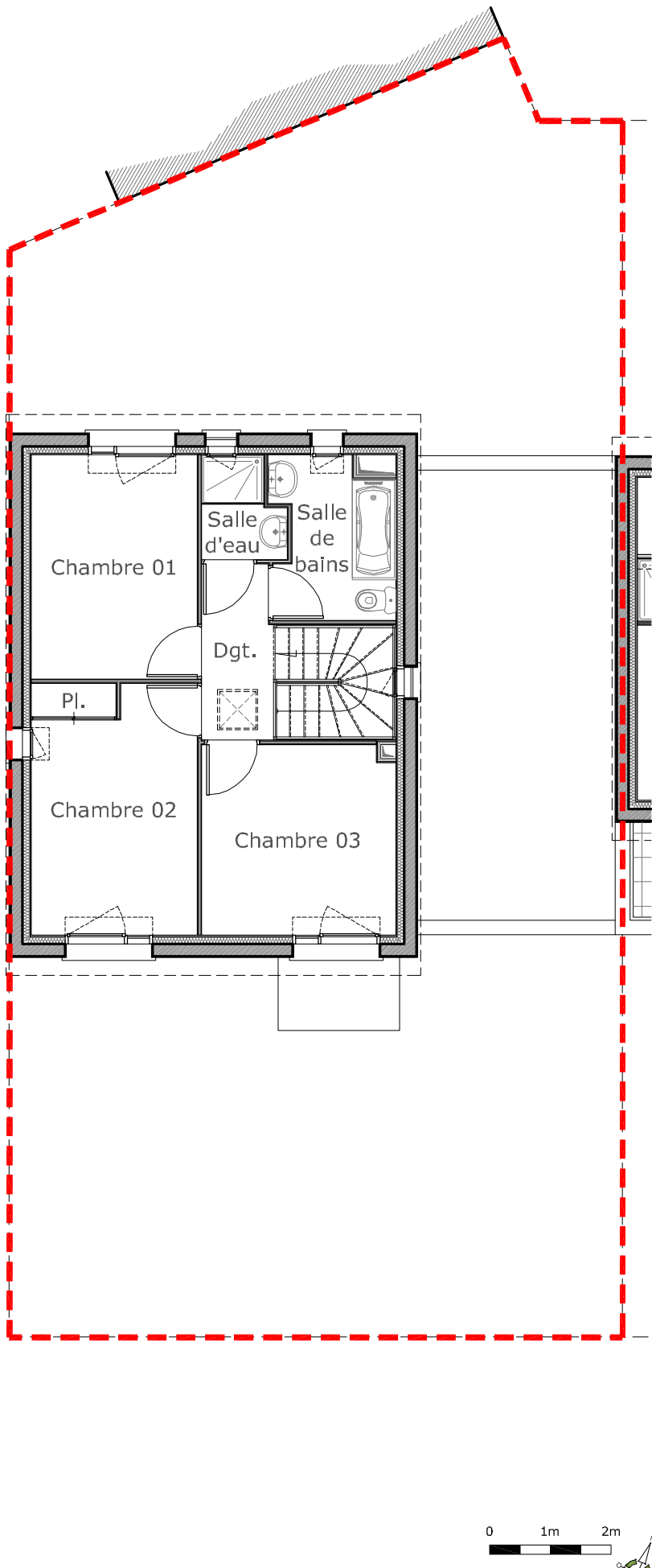
Plan R+1
